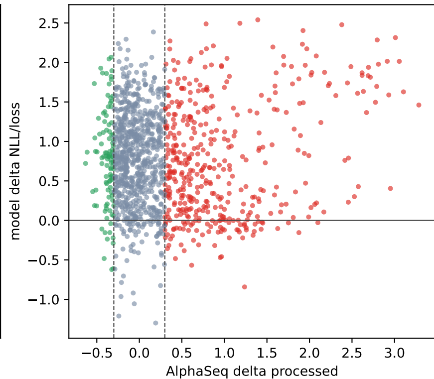
Weighted
